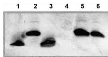
Fig. 5. Interaction between importin \alpha -GST and oligonucleotide-NLS peptide conjugates. Immobilized importin \alpha -GST (2 \mu g) was incubated for 30 min at room temperature with Pso-GA 19 (2 \mu g) (lanes 3 and 4), Pso-GA 19 -NLS (lanes 5 and 6). Free Pso-GA 19 (lane 1), free Pso-GA 19 -NLS (lane 2) and fractions bound to importin \alpha -GST (lanes 4 and 6) and unbound (lanes 3 and 5) were analyzed by 15% denaturing polyacrylamide gel electrophoresis and silver staining.
